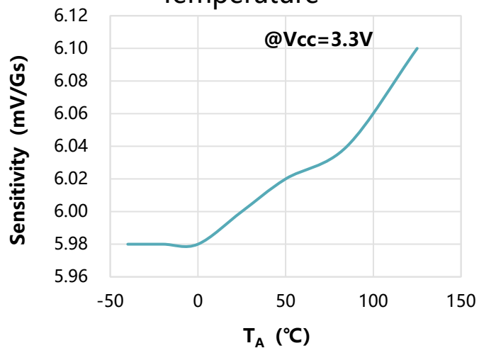
Sensitivity versus Ambient Temperature
