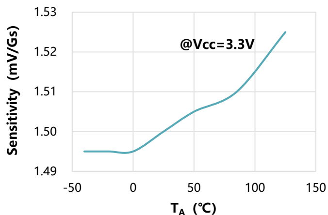
Sensitivity versus Ambient Temperature
